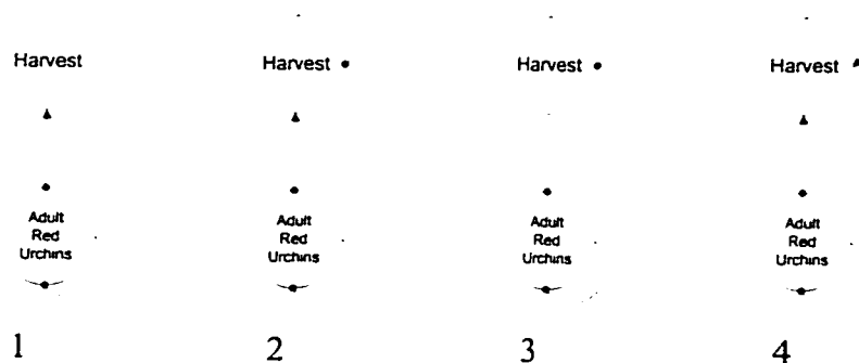
Figure 5.2. Fishery scenarios described by Dambacher ( personal communication ) tested to identify the models from the harvested areas: 1) artisanal harvest (obligate predator), 2) well managed fishery (quota \leq MSY), 3) modern fishery where perfect quota is in equilibrium with community (right at MSY), and 4) fishery with fixed quota > MSY.
