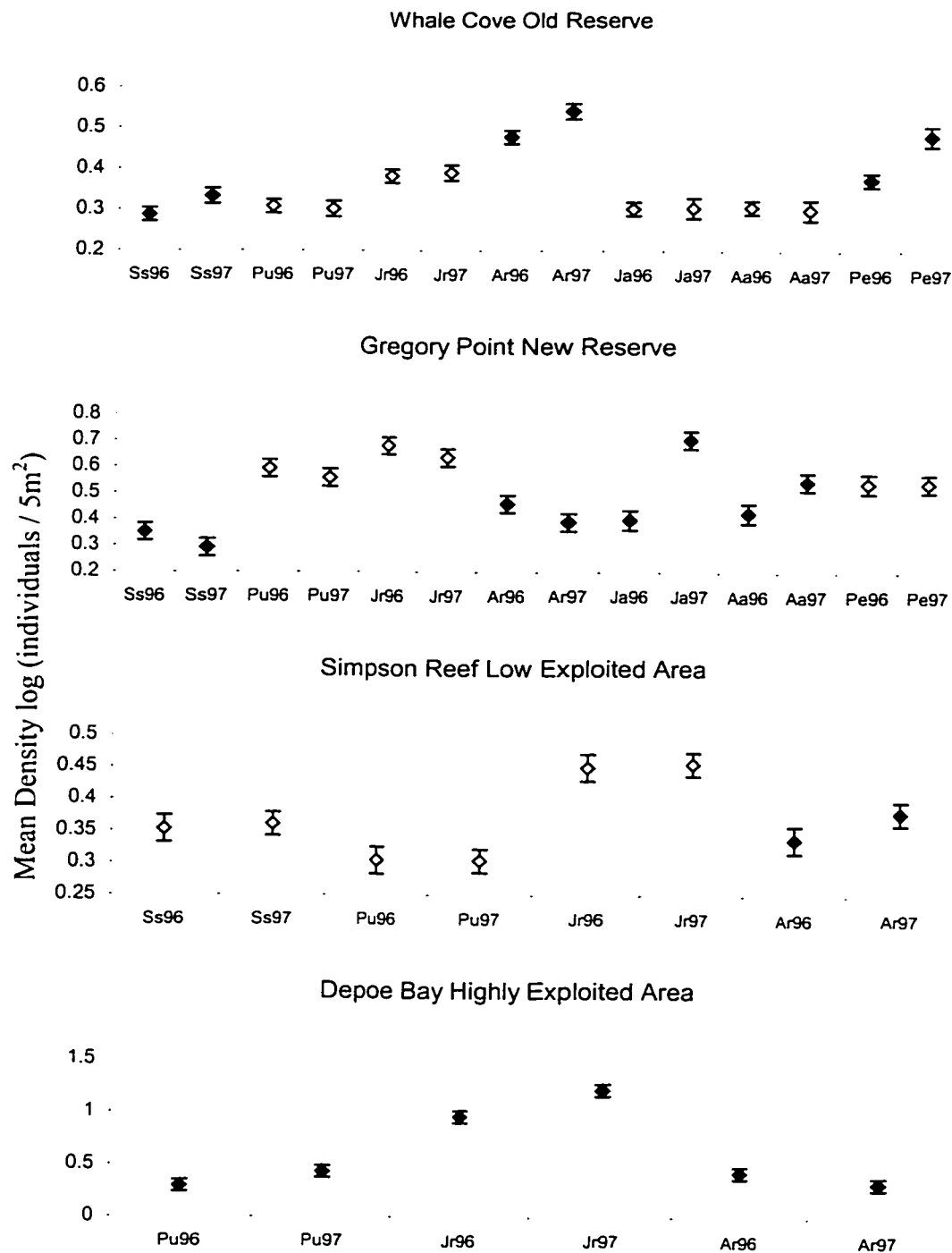
Figure 5.3. Changes in mean density of each species over two consecutive years (1996-1997) in two reserves and adjacent exploited areas. Significant changes are indicated as black triangles and non-significant changes as white triangles. Ss = sunflower stars, Pu = purple urchins, Jr = juvenile red urchins, Ar = adult red urchins, Ja = juvenile annual kelp, Aa = adult annual kelp, and Pe = perennial kelp. Standard error bars are indicated.
