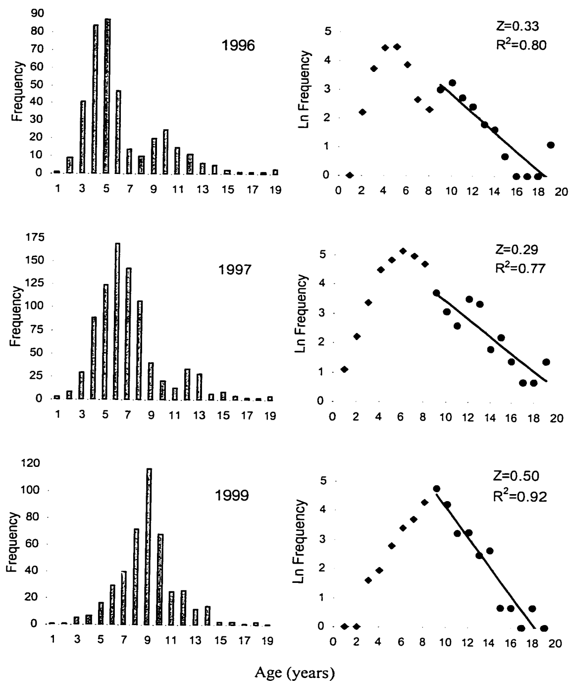
Figure 3.10. Red urchins age distribution for Gregory Point marine reserve between 1996 and 1999. Catch curve analyses for each year are indicated on the right panel. The slope of the descending part of the curve corresponds to the natural mortality rate (M). In a reserve, total mortality (Z) is equal to natural mortality (M).
