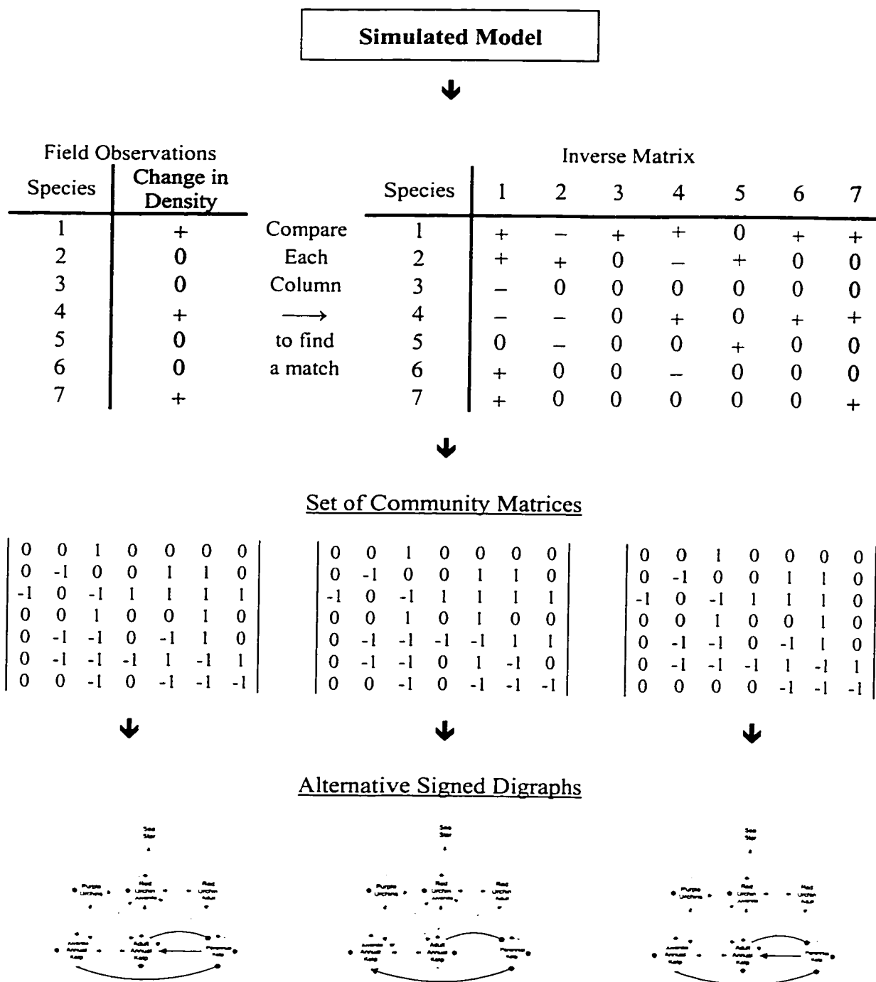
Figure 4.3. Qualitative simulation procedure to obtain the models that best represent the community structure from Whale Cove. Shaded areas indicate the column that matched the observations, which is the variable (species 7) where the disturbance entered the system. The inverse matrix (prediction matrix) shows the predictions about the effect (+, -, 0) on equilibrium abundances for each species when a disturbance causes a parameter change in all variables. Changes in species abundance from year to year are assumed to be in response to a disturbance to the system. Therefore, they correspond to predictions from the inverse matrix.
