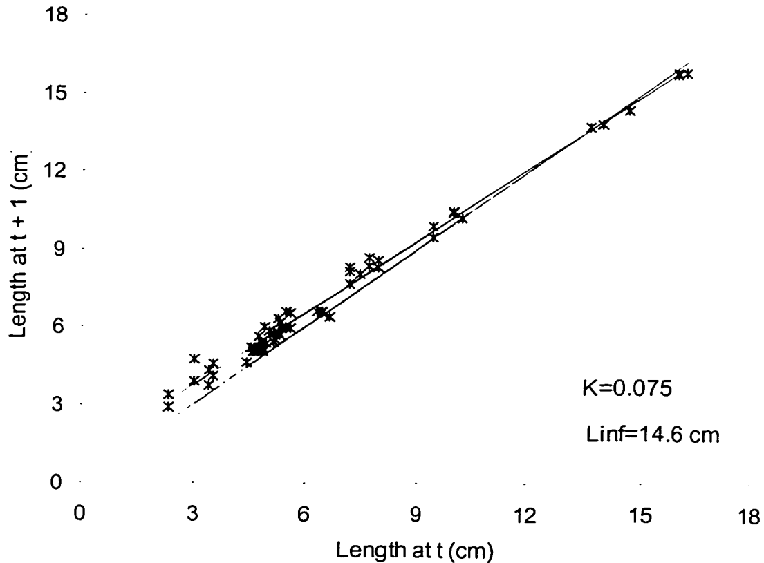
Figure 3.2. Ford-Waldford plot of red urchins reared in laboratory conditions for 1 year. Regression: y = 0.97 + 0.93x ; K = -\ln 0.93 = 0.075 ; L_{\infty} = 14.6 cm. Dashed line = no growth.
