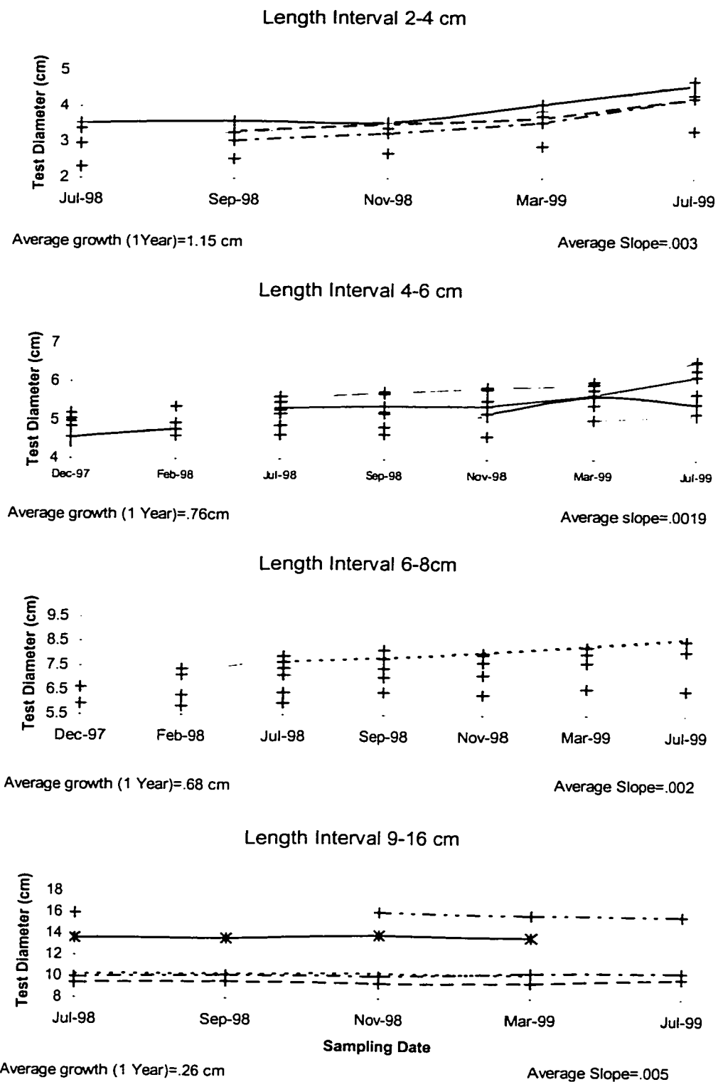
Figure 3.1. Changes in length through time for different length intervals of red urchins reared in laboratory conditions. Each line represents an individual.
